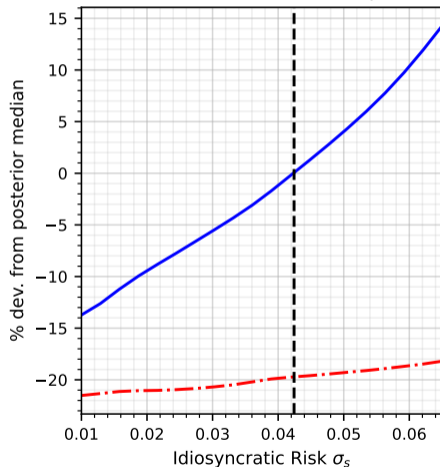
Standard Deviation of Output \tilde{Y}
